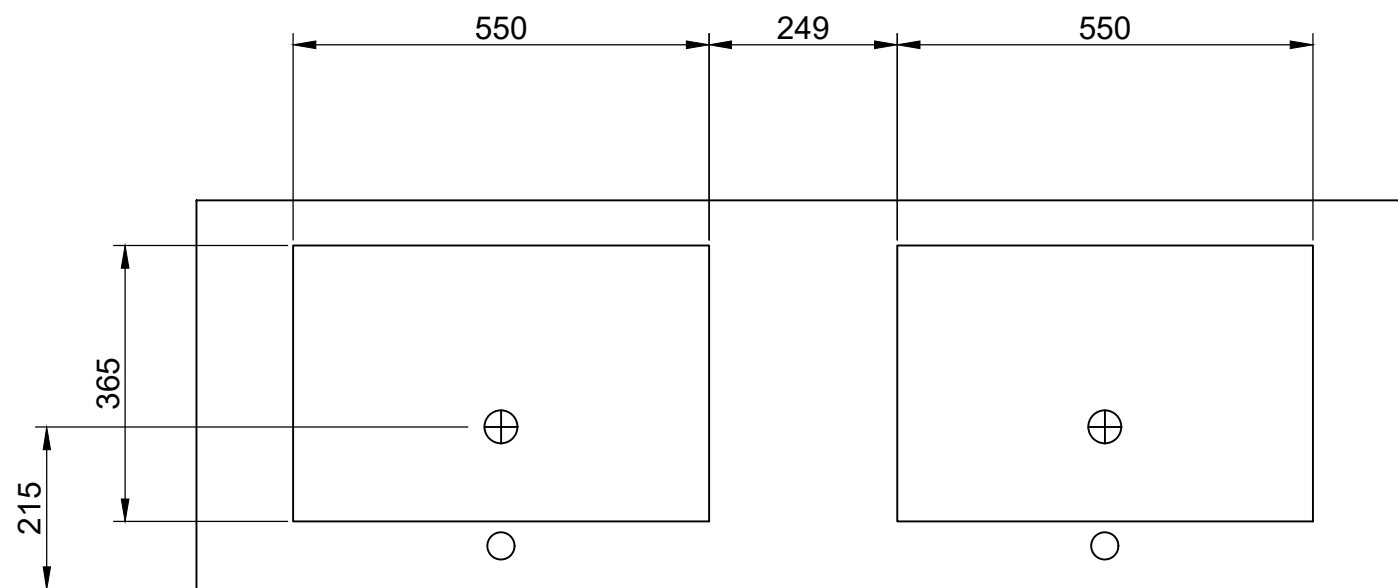
BOTTOM VIEW
