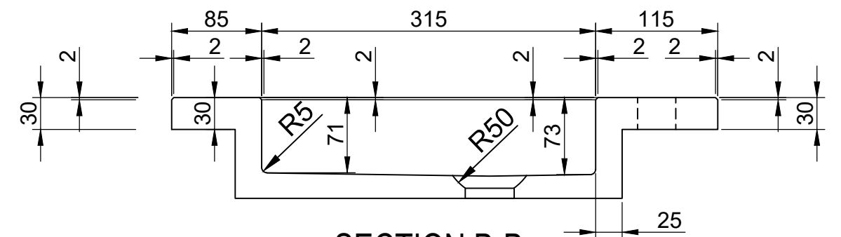
SECTION B-B SCALE 1:5
